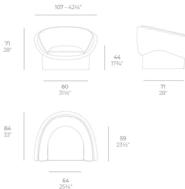
LUNA Butaca LUNA Armchair ref. 54850
