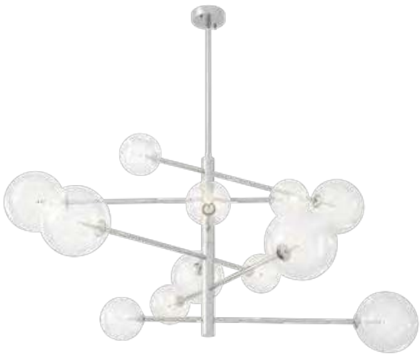
Chandelier Argento L Nickel finish | clear glass ø 130 x H. 67 cm 111975 Lamp holder: 12 x G4 I max. 10 watt
